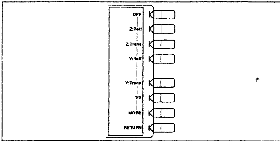
Figure 9-5A. Conversion Menu
