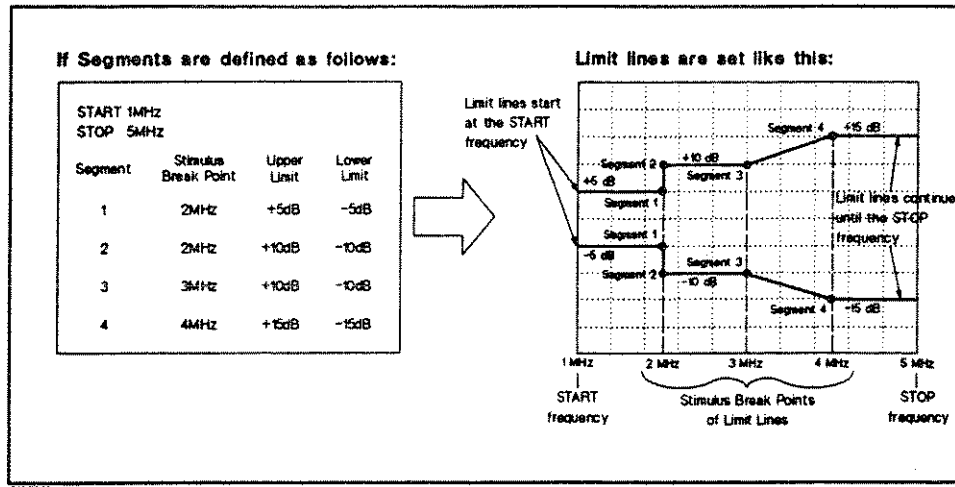
Figure 12-16. The Concept of Segments as a Point between Two Sets of Limit Lines
