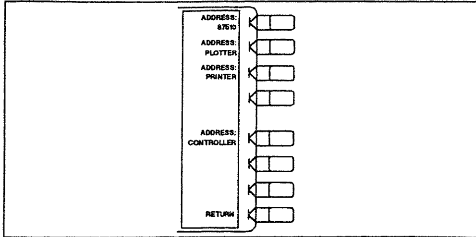
Figure 12-4. Address Menu
