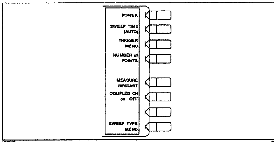
Figure 8-3. Stimulus Menu
