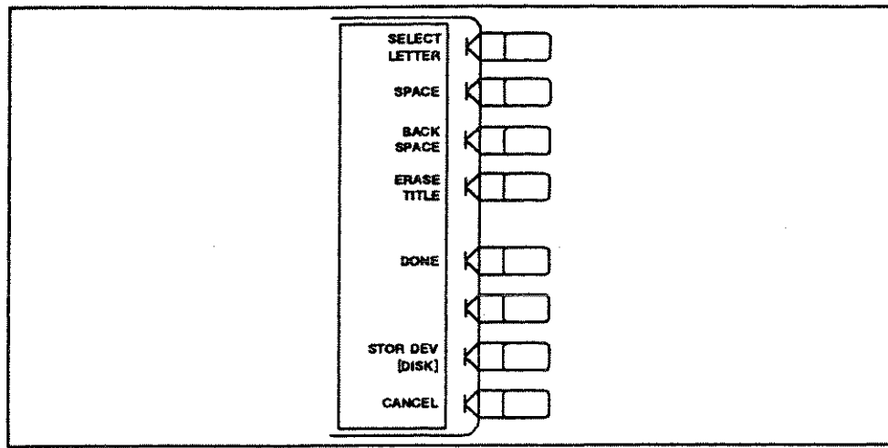
Figure 14-17. Destination Menu
